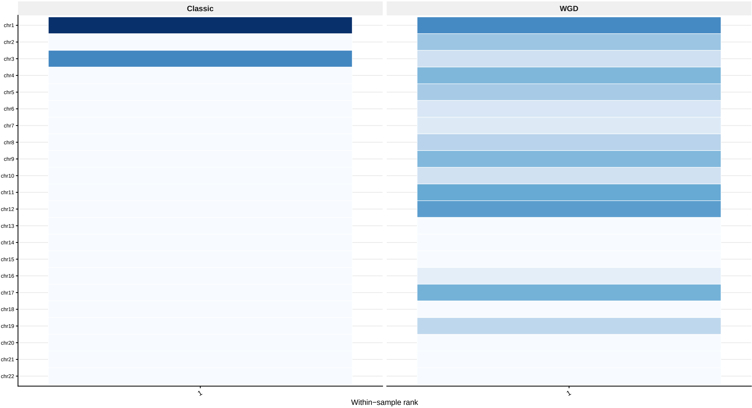
Chromosome coverage density by class × clock rank Colour = sum(seg length) / chr length / n_samples | Stars = Wilcoxon vs row median (BH)
